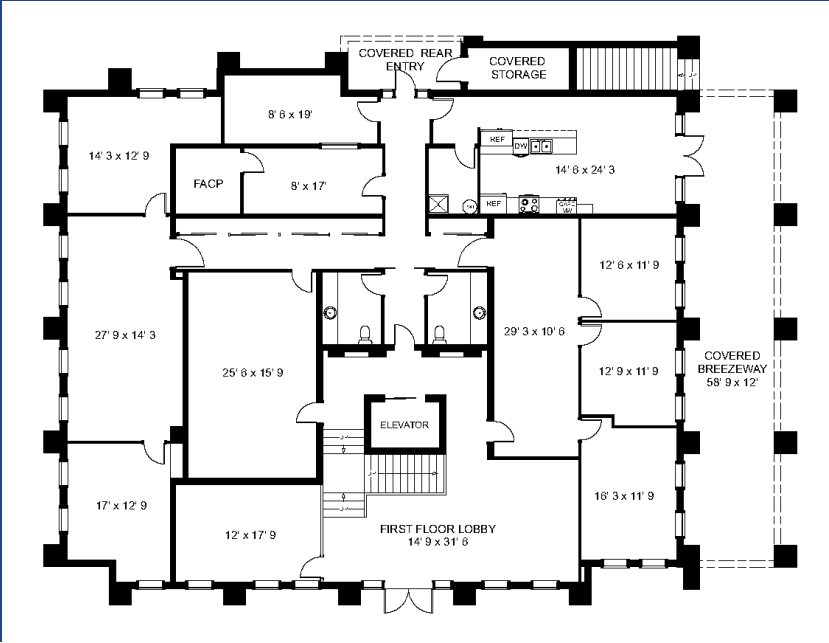
1 st Floor
