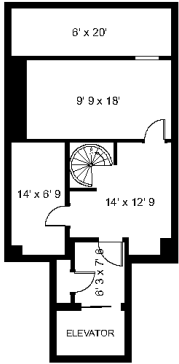
3 rd Floor
